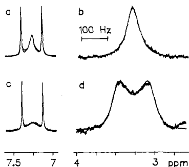
Figure 2. Superposed experimental and calculated 300.13 MHz ^1\text{H} NMR spectra of a 0.1 M solution of 1 in methylcyclohexane- d_{14} (MCY) at 362 K: (a) ^{15}\text{N} - ^1\text{H}\cdots^{15}\text{N} signal of Ia-HH and (b) 4,4' and 7,7' proton signal of Ib-HH at a deuterium fraction D = 0 in the mobile proton sites; (c) ^{15}\text{N} - ^1\text{H}\cdots^{15}\text{N} signal of Ia-HD, and (d) 4,4' and 7,7' proton signal of Ib-DD at a deuterium fraction D = 0.94 in the mobile proton sites (200–1800 scans on average, 60^\circ pulses, 3s repetition time, 2500 Hz sweep width, 16 K spectra). The presence of a small amount of 1c was taken into account in the simulations; in addition, at D = 0.94 the presence of Ia-HH, Ib-HH, and Ib-HD was also taken into account. Simulation parameters: a, b, k^{\text{HH}} = 635 \text{ s}^{-1} ; c, k^{\text{HD}} = 260 \text{ s}^{-1} ; d, k^{\text{DD}} = 215 \text{ s}^{-1} . Further simulation parameters: \nu_{\text{H-}^{15}\text{N}} = 7.26 \text{ ppm} , ^1J_{\text{H-}^{15}\text{N}} = 80.3 \text{ Hz} , W_0 = 3.7 \text{ Hz} , and chemical shifts \nu_4 = \nu_{4'} = 3.505 \text{ ppm} and \nu_7 = \nu_{7'} = 3.03 \text{ ppm} . For further description see text.
