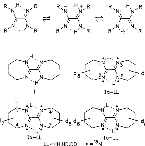
Figure 1. The stepwise double-proton-transfer in oxalamidine (OA, R = H), tetraphenylloxalamidine (TPOA, R = phenyl), 6 and I. 29
