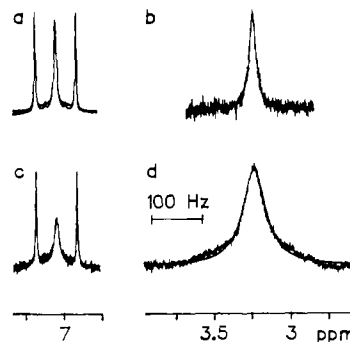
Figure 3. Superposed experimental and calculated 300.13 MHz ^1\text{H} NMR spectra of a 0.1 M solution of 1 in acetonitrile- d_3 (AN) at 362 K: (a) ^{15}\text{N} - ^1\text{H}\cdots^{15}\text{N} signal of Ia-HH and (b) 4,4' and 7,7' proton signal of Ib-HH at a deuterium fraction D = 0 in the mobile proton sites; (c) ^{15}\text{N} - ^1\text{H}\cdots^{15}\text{N} signal of Ia-HD, and (d) 4,4' and 7,7' proton signal of Ib-DD at a deuterium fraction D = 0.94 in the mobile proton sites. Simulation parameters: a, b, k^{\text{HH}} = 2870 \text{ s}^{-1} ; c, k^{\text{HD}} = 1090 \text{ s}^{-1} ; d, k^{\text{DD}} = 830 \text{ s}^{-1} . Further simulation parameters: \nu_{\text{H-}^{15}\text{N}} = 7.05 \text{ ppm} , ^1J_{\text{H-}^{15}\text{N}} = 80.3 \text{ Hz} , W_0 = 3 \text{ Hz} , and chemical shifts \nu_4 = \nu_{4'} = 3.492 \text{ ppm} and \nu_7 = \nu_{7'} = 2.965 \text{ ppm} . For further description see Figure 2 and text.
